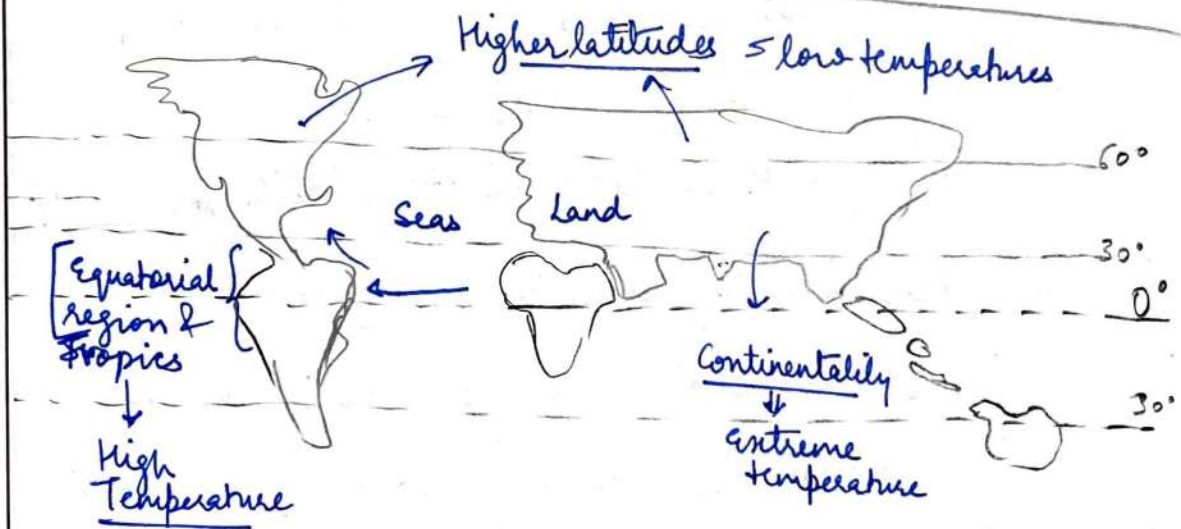
* Fig : Temperature Distribution on World
