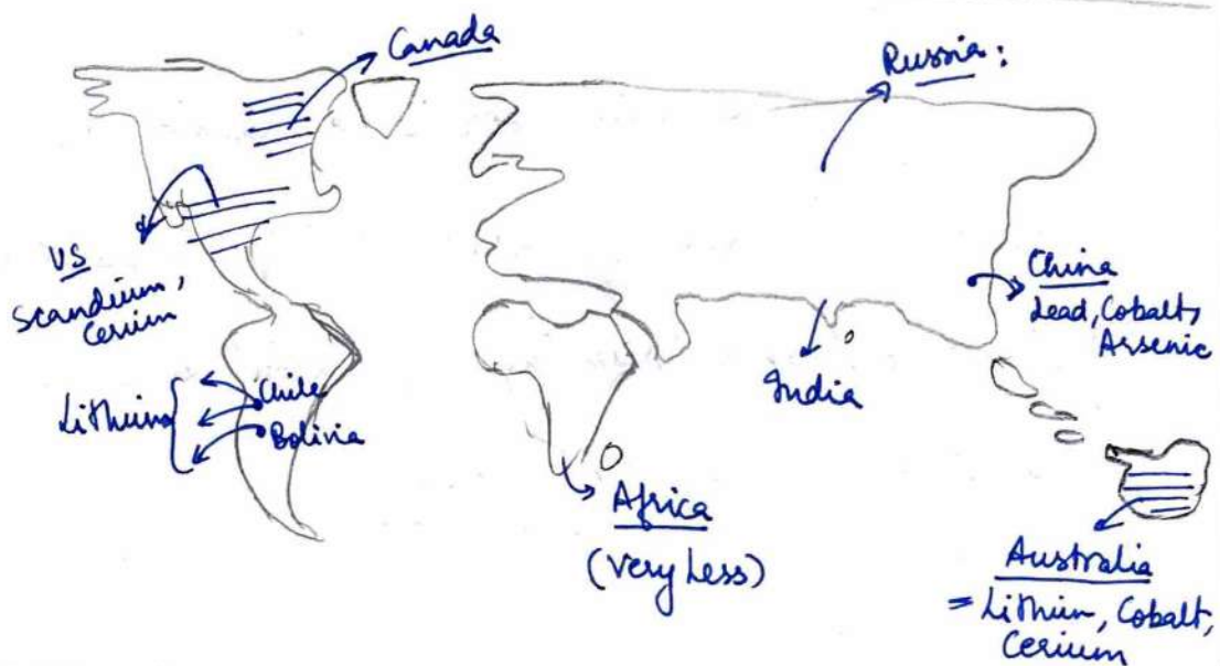
* Fig : Distribution of Rare Earth Elements
